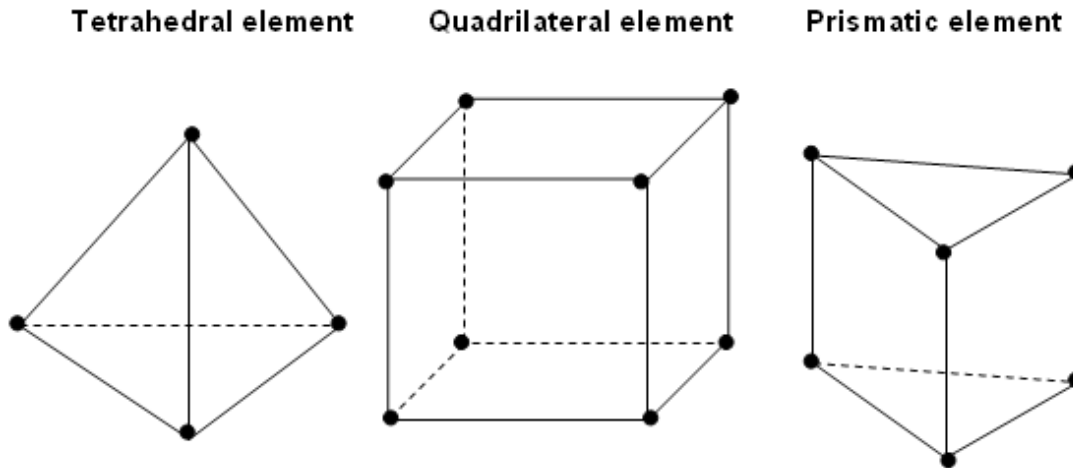
Figure 6-11: Three-dimensional elements
